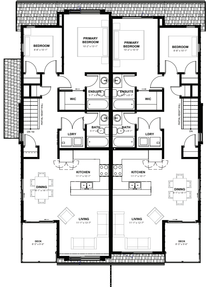
2nd floor 1012 SQ.FT. | 988 SQ.FT.
