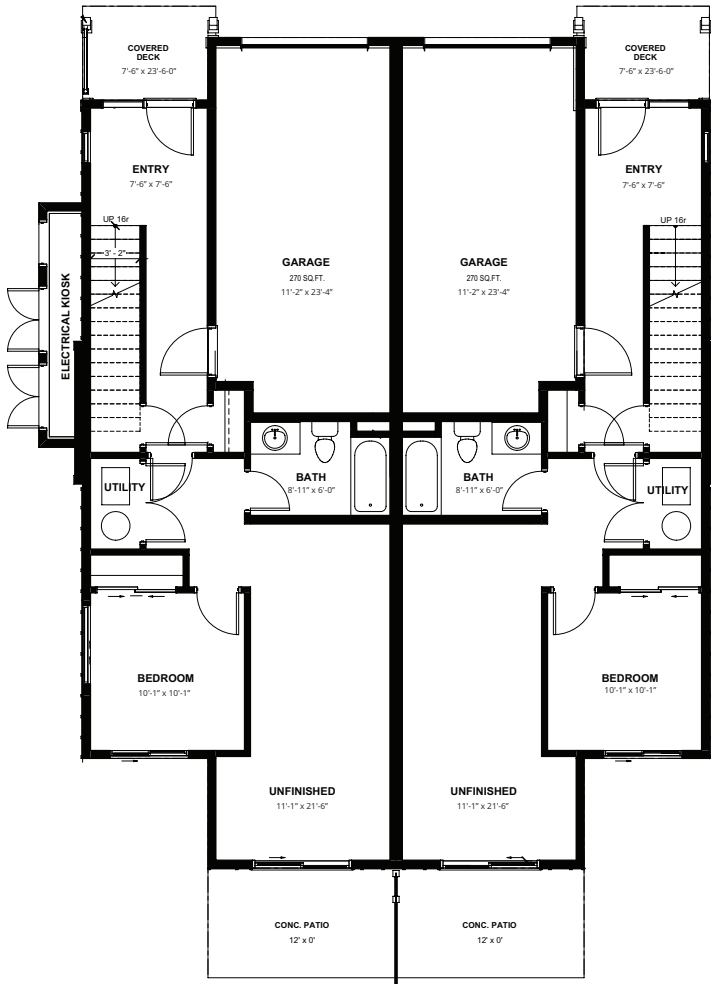
main floor 694 SQ.FT. | 694 SQ.FT.
