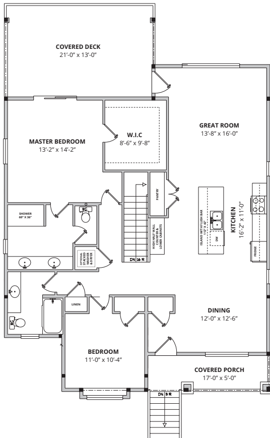
main floor 1,446 SQ.FT.
