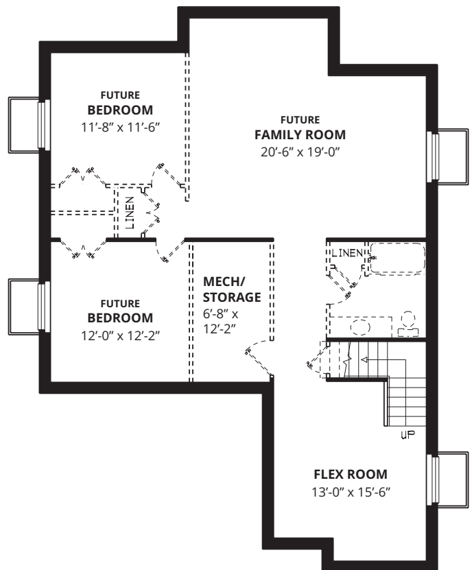
basement 1,299 SQ.FT.
